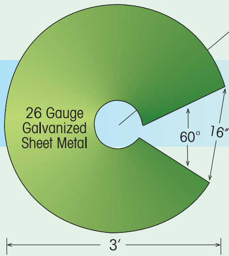
CONE GUARD
